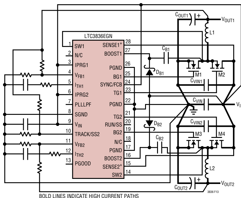
Figure 13. LTC3836 Layout Diagram
