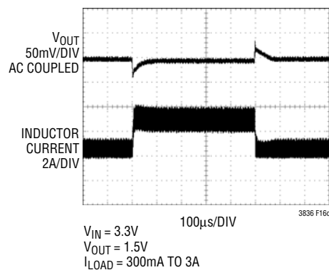
Figure 16c. Load Step
