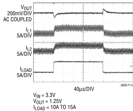
Figure 17c. Load Step
